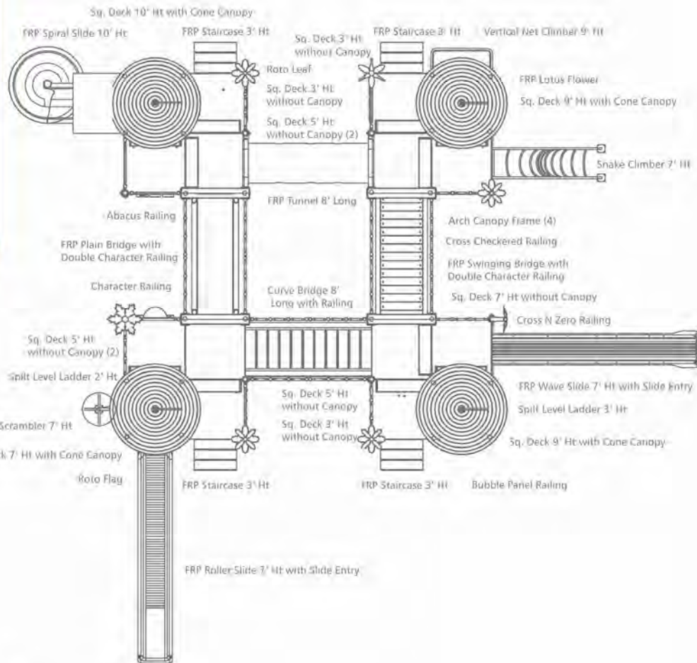
Technical Layout: Theme M.A.P.S: T 34
