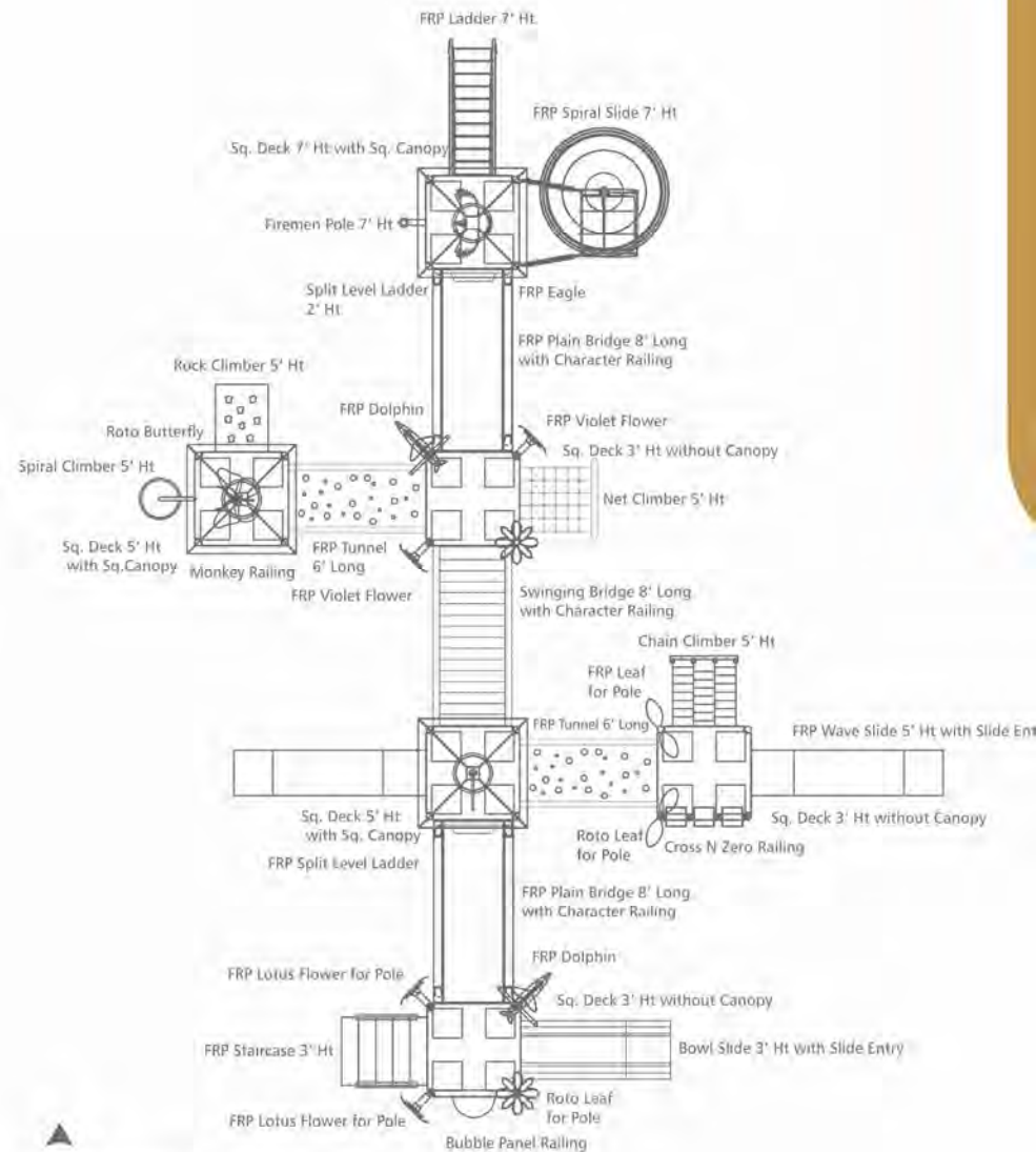
Technical Layout: Theme M.A.P.S: T 03
